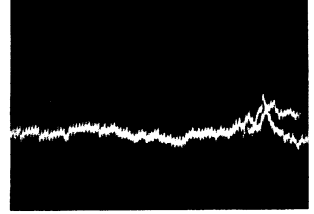
TP SPD (Spindle out) Vertical : 1V/div. Horizontal : 5 ms/div. DC, Ground: Center
